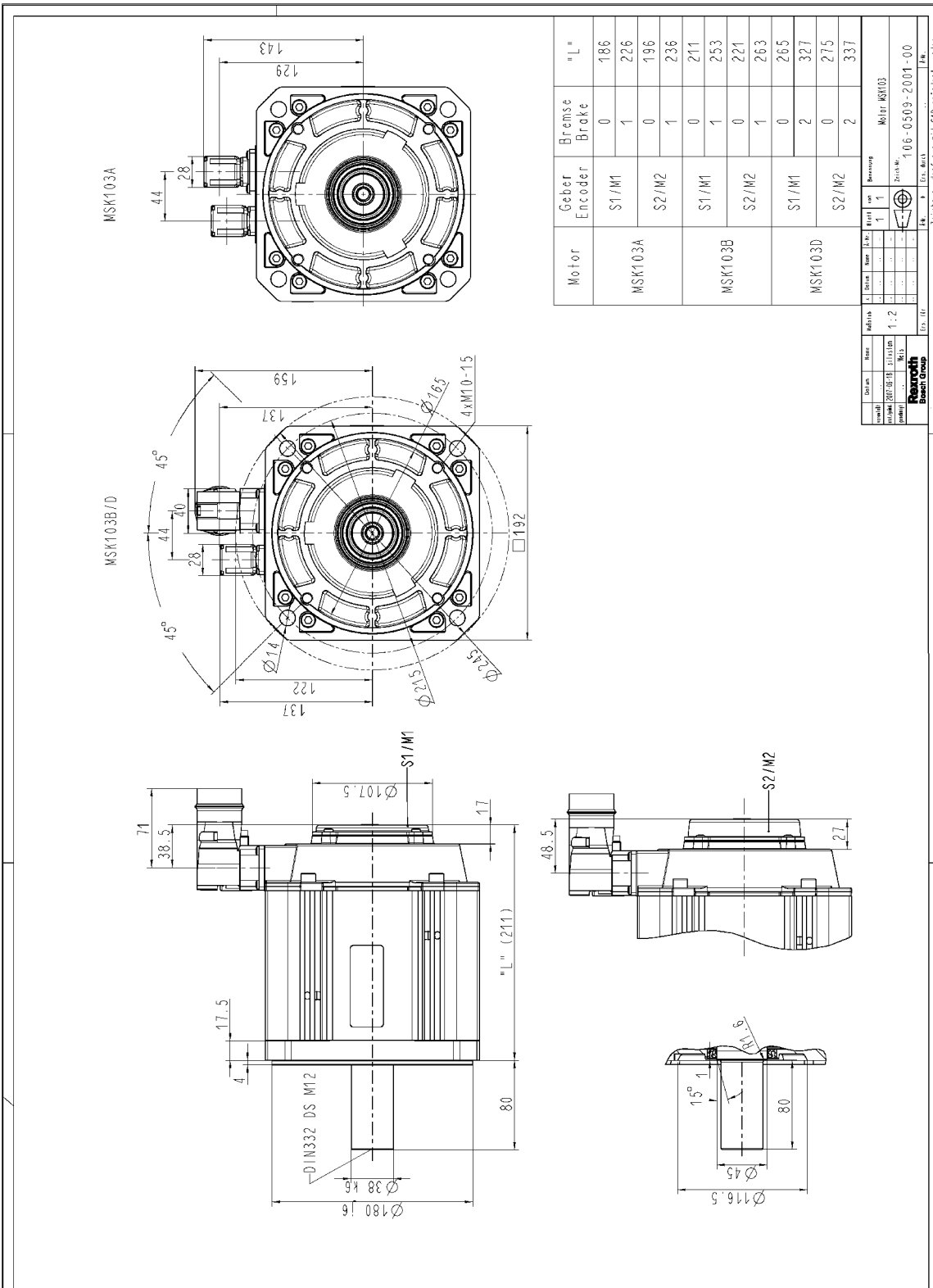
Fig.5-17: MSK103 specification
