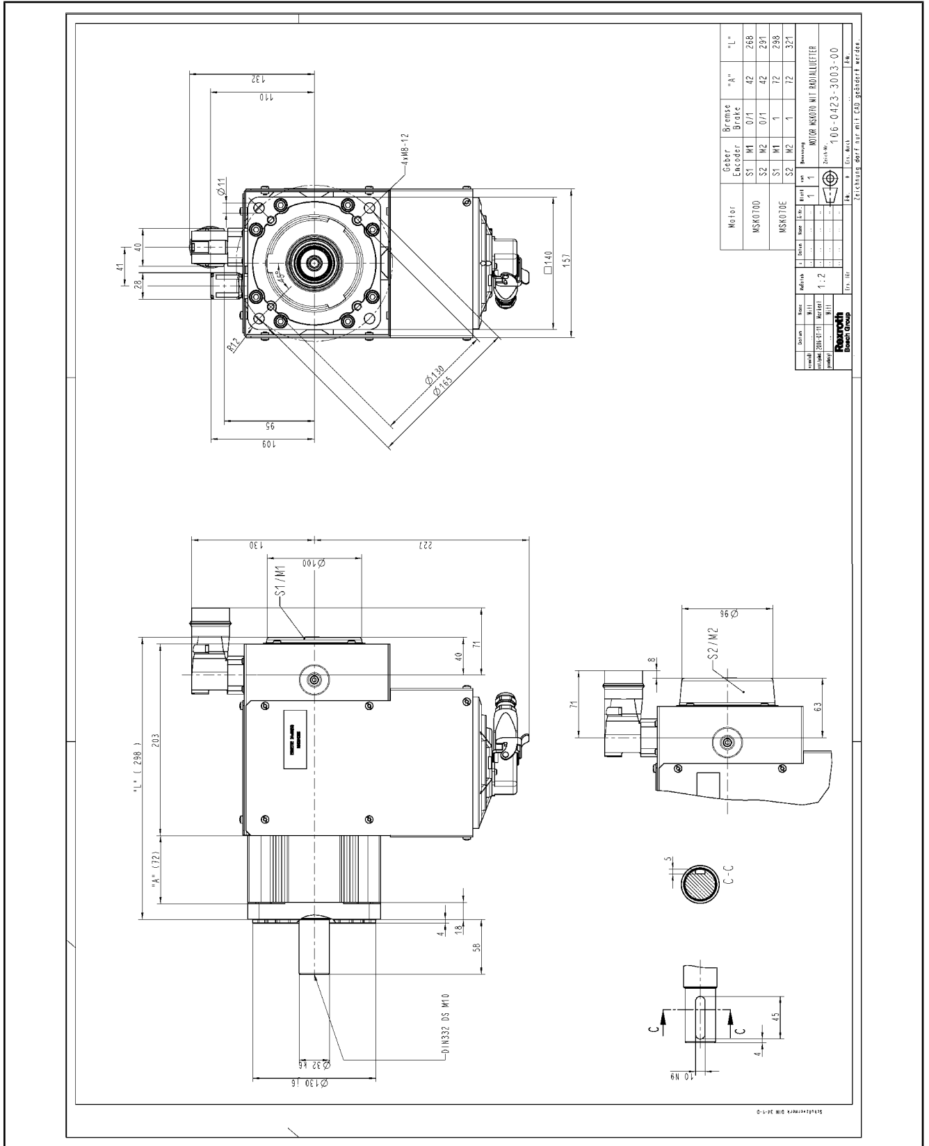
Fig.7-12: Dimension sheet MSK070 with radial fan unit
