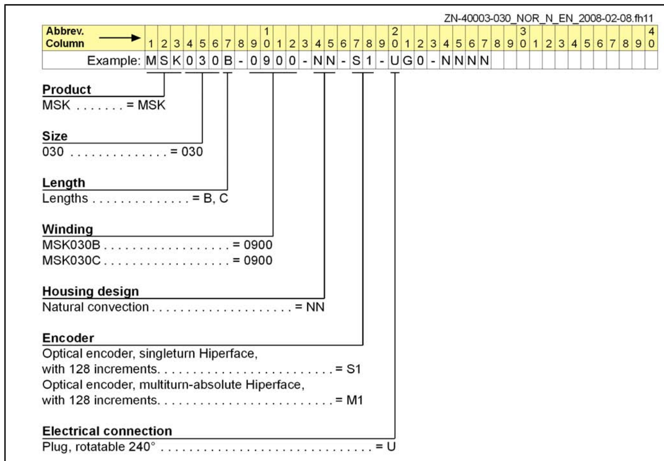
Fig.6-6: MSK030 type code (page 1)
