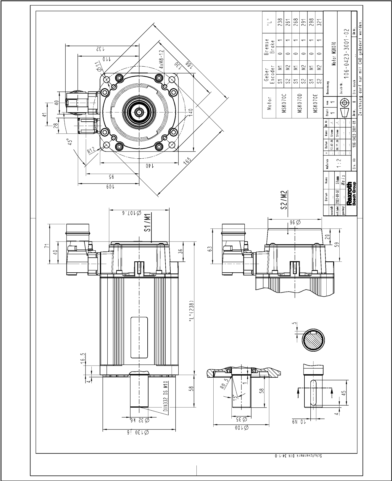
Fig.5-8: MSK070 specification
