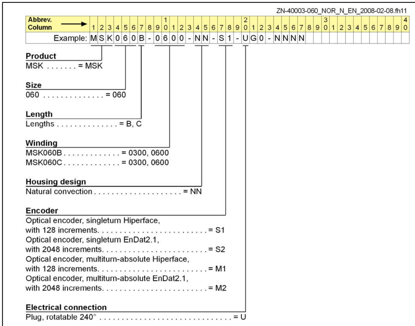
Fig. 6-12: MSK060 type code (page 1)
