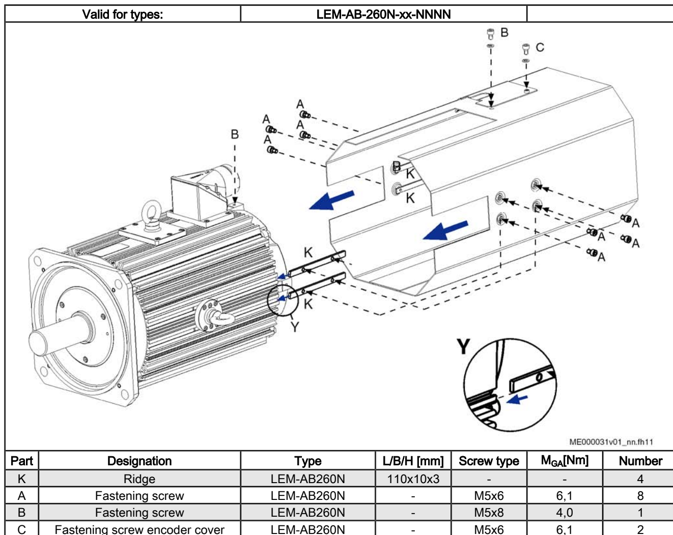
Fig.7-28: Assembly Fan Unit Axial, Flange Dimension 260
