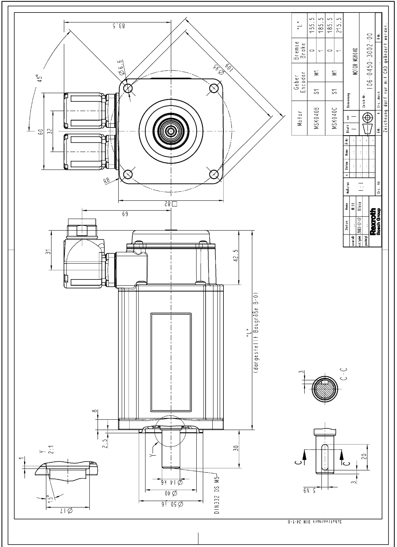
Fig.5-4: MSK040 specification
