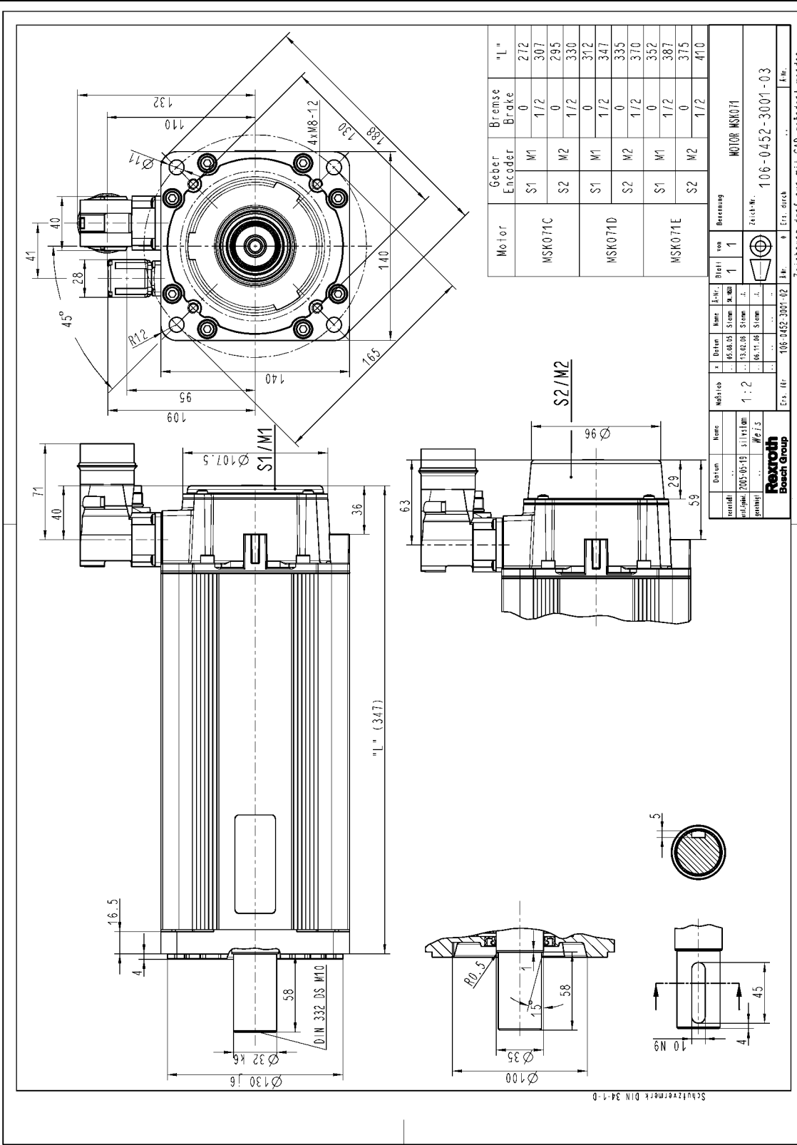
Fig.5-9: MSK071...NN specification
