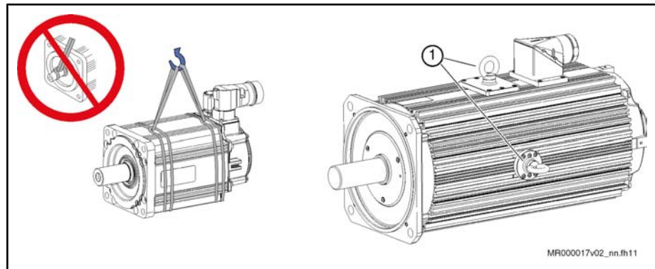
Fig. 10-4: Lifting and transporting motors by means of lifting sling belts
