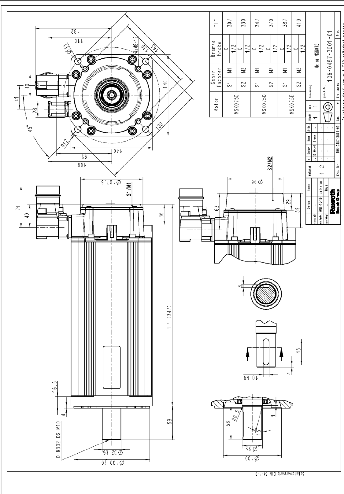
Fig.5-11: MSK075...NN specification
