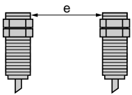
Mounting side by side e \geq 0.3 at 3 m
